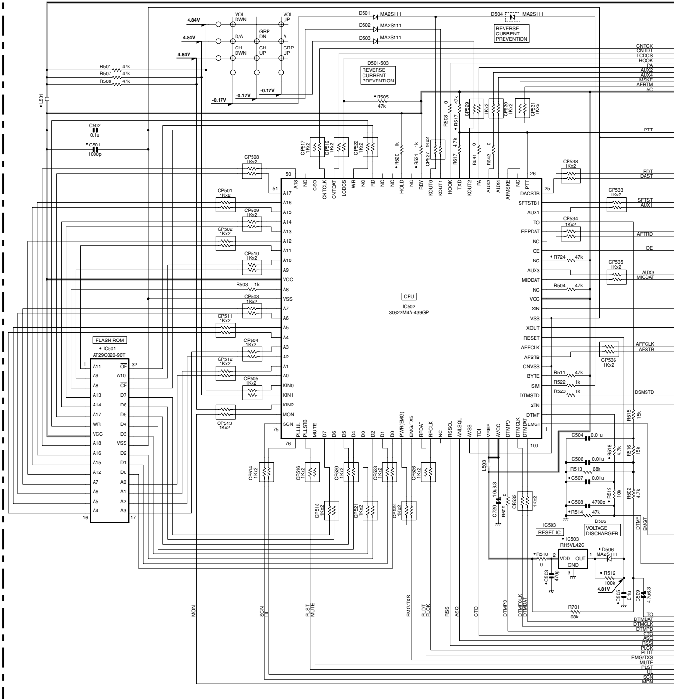
CONTROL UNIT (X57-5963-01) (B/2)
