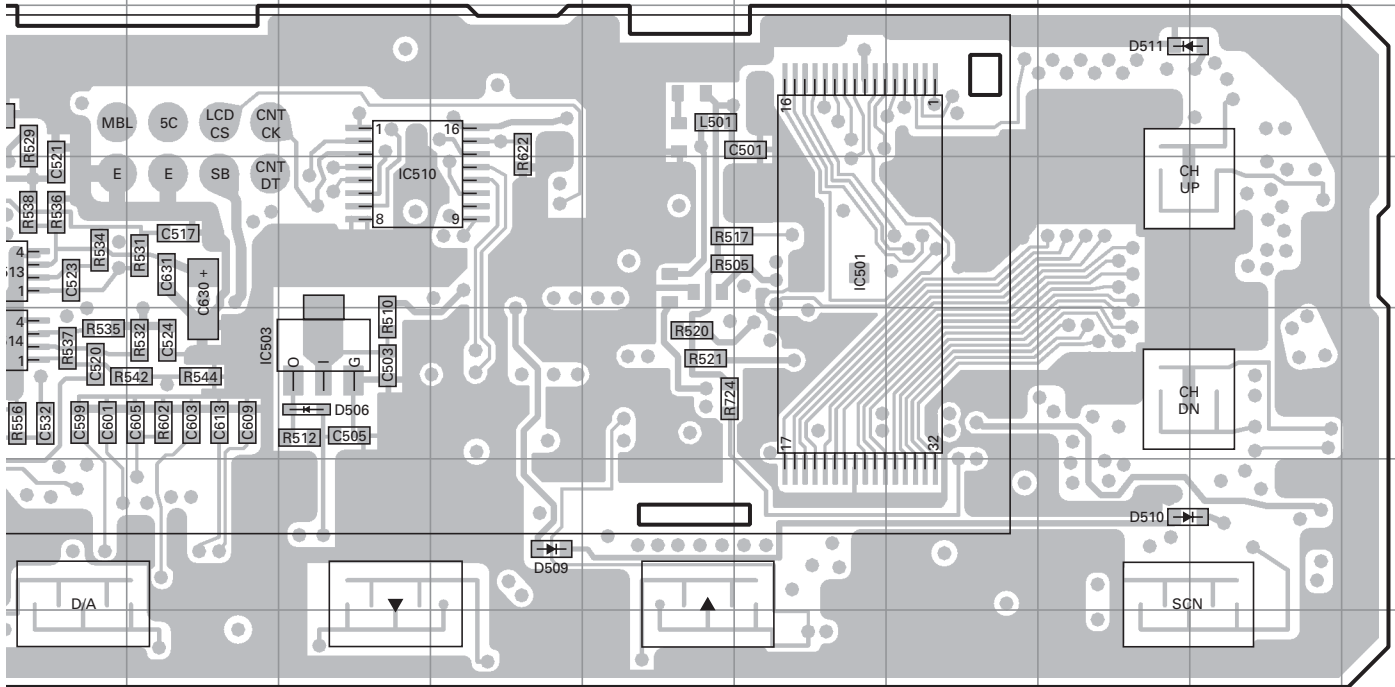
TX-RX UNIT (X57-5963-01) (B/2) Component side view (J72-0988-09 B/2)
