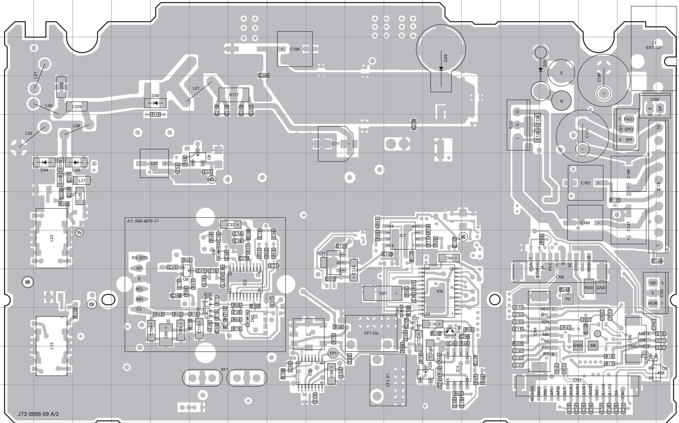
TX-RX UNIT (X57-5963-01) (A/2) Component side view (J72-0988-09 A/2)
