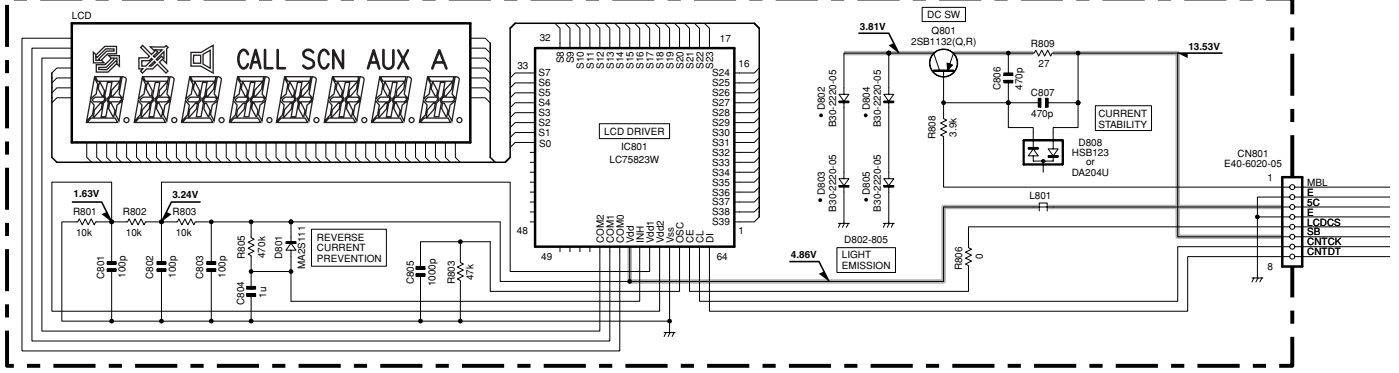
CONTROL UNIT (X57-5963-01) (B/2)
