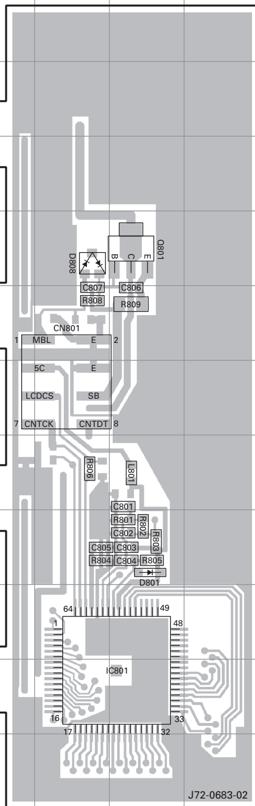
DISPLAY UNIT (X54-3270-10) Foil side view (J72-0683-02)
