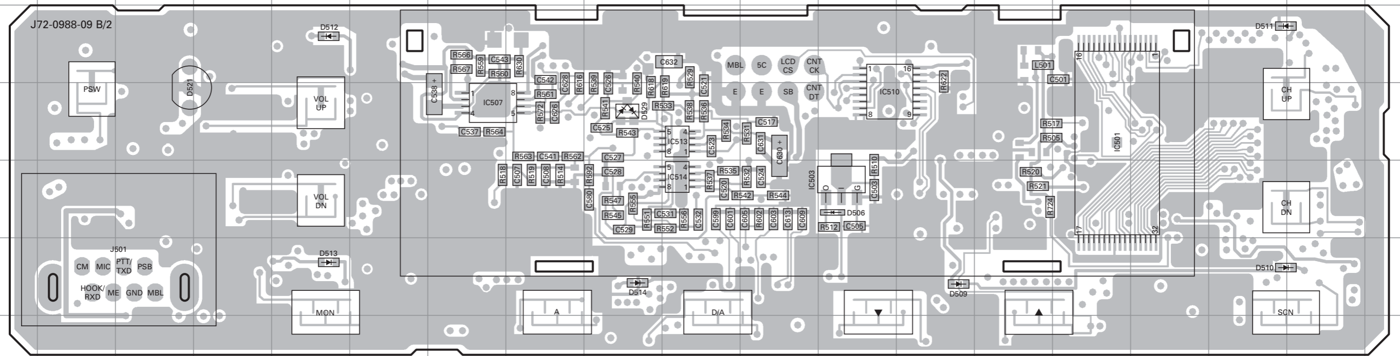
TX-RX UNIT (X57-5963-01) (B/2) Component side view (J72-0988-09 B/2)
