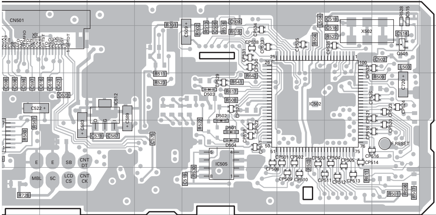
TX-RX UNIT (X57-5963-01) (B/2) Foil side view (J72-0988-09 B/2)
