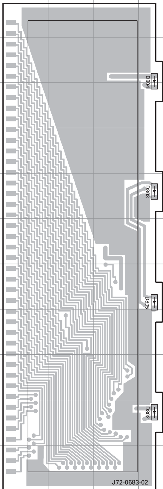
DISPLAY UNIT (X54-3270-10) Component side view (J72-0683-02)
